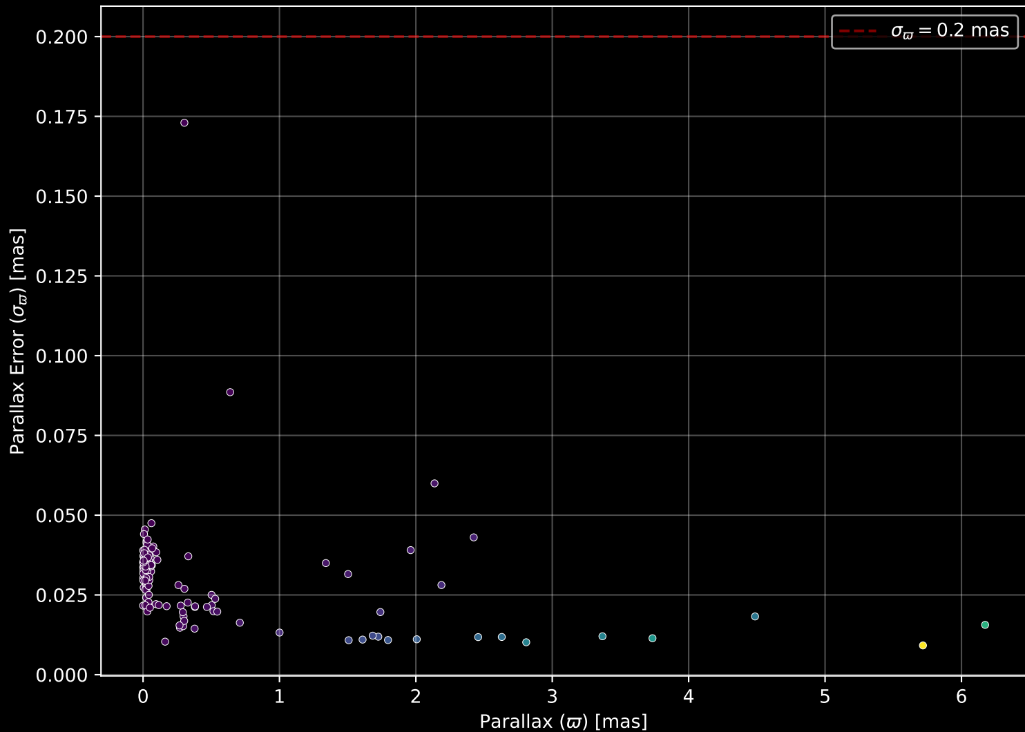
APOGEE DR17 Field: [SMC4] Parallax Quality (n= 152)
