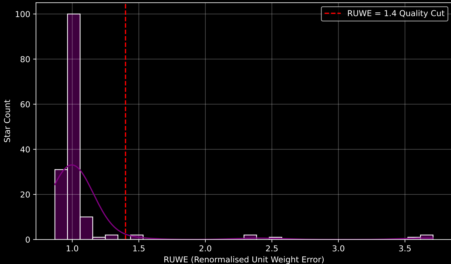
GAPOGEE DR17 Field [SMC4] RUWE Distribution (n= 152)
