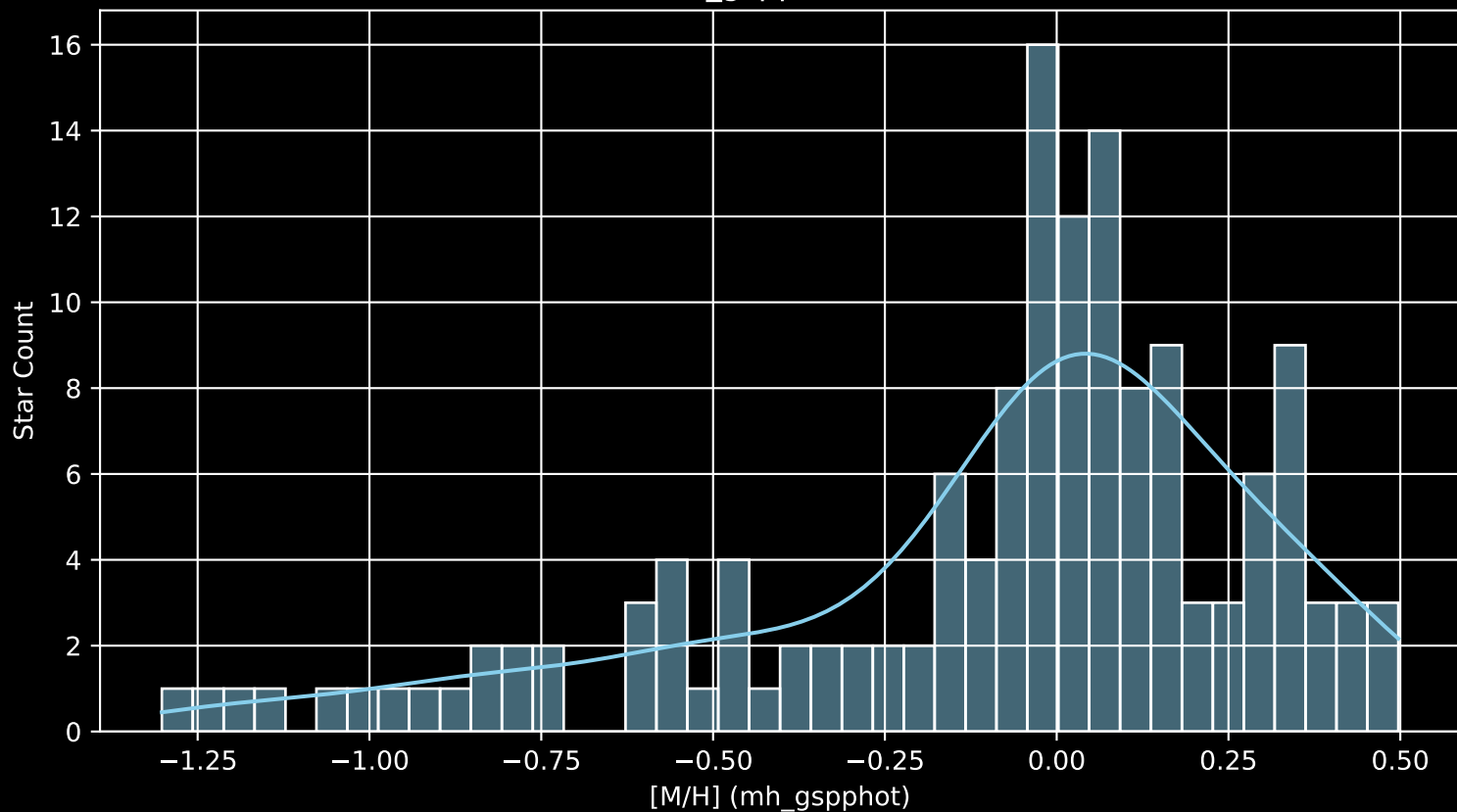
APOGEE DR17 Field: [SMC4 [M/H] (mh_gspphot) (n= 145)
